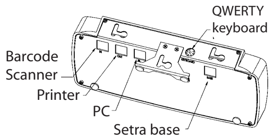
Controller Ports
