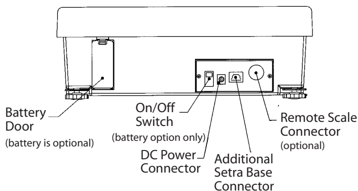
Setra Base - Rear View
