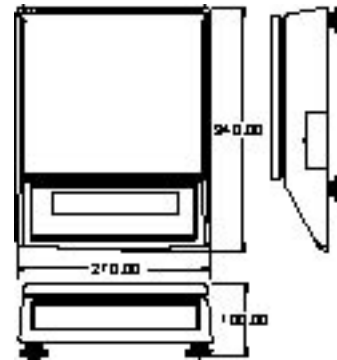
OUTLINE OF SCALE AND DIMENSIONS
